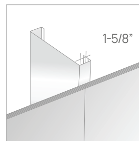
Minimum 1-5/8" wide
